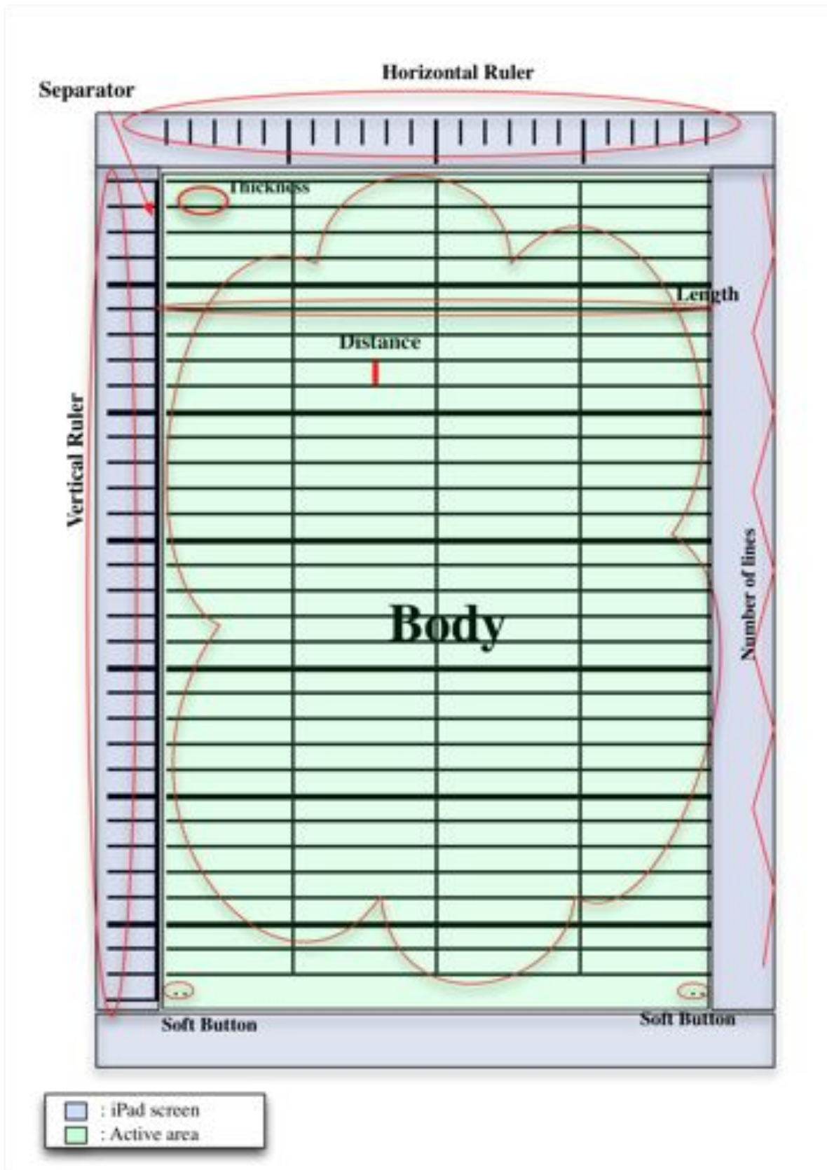
Figure 3.5: Illustration of the different elements of the overlay.
